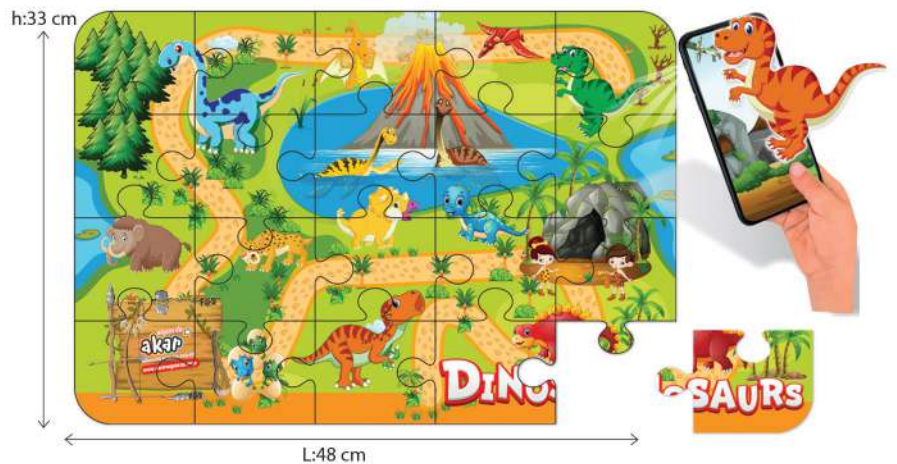
Augmented Reality
